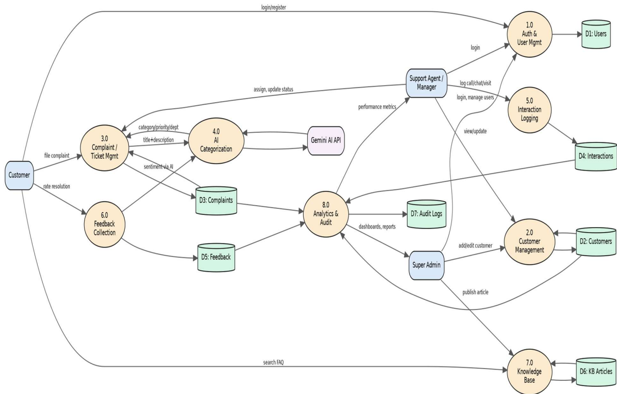
Figure 2: Level-1 DFD — core sub-processes and data stores
